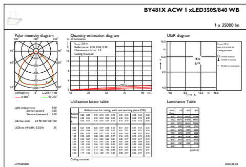
IFGU1_BY481XACW1xLED350S840WB
