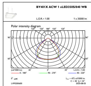
OFPC1_BY481XACW1xLED350S840WB
