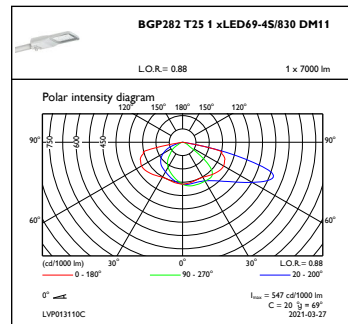
OFPC1_BGP282T251xLED69-4S830DM11
