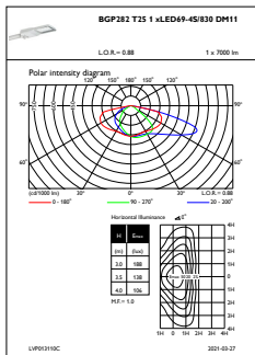
OFPL1_BGP282T251xLED69-4S830DM11
