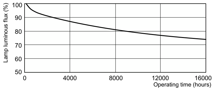
Lumen Maintenance Diagram - MASTER TL5 Circular 40W/840 1CT/10
