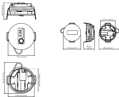
EasyAir SNS401CMP
