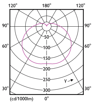
LEDTForce Core 35W Tshape E27
