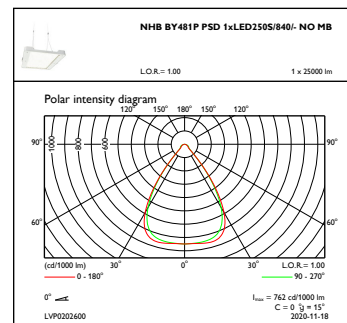
OFPC1_BY481PPSDHE1xLED250S840MB
