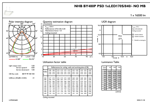
IFGU1_BY480PPSDHE1xLED170S840MB
