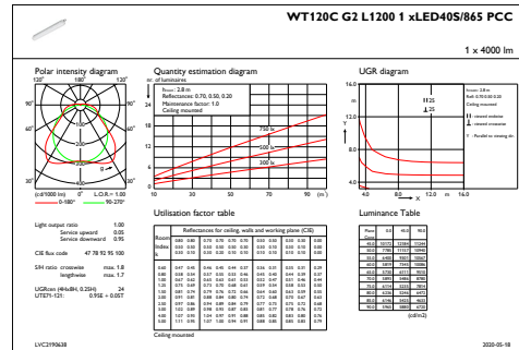
IFGU1_WT120CG2L12001xLED40S865PCC
