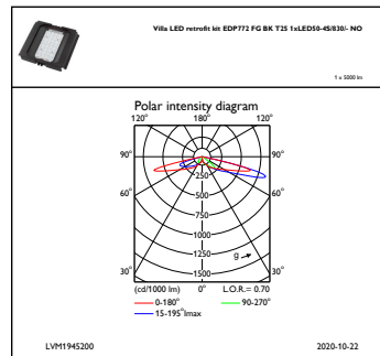
IFPC1_EDP772FGBKT251xLED50-4S830DM50
