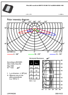
OFPL1_EDP772FGBKT251xLED50-4S830DM50
